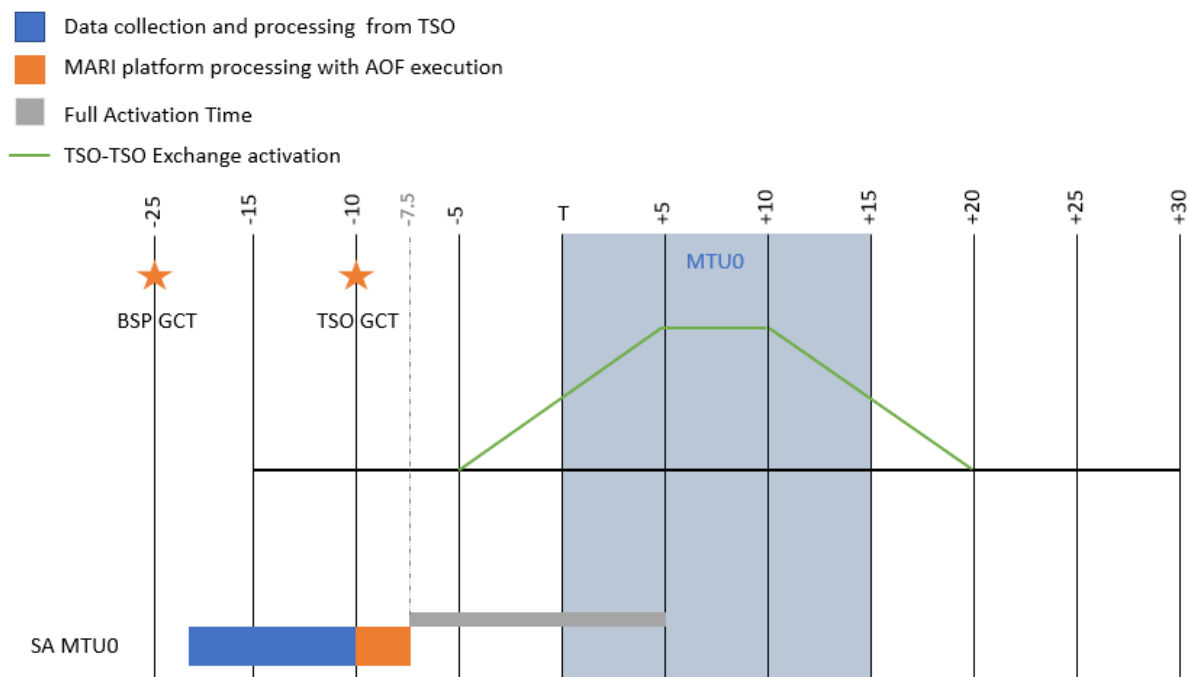
Figure 3: Scheduled Activations
