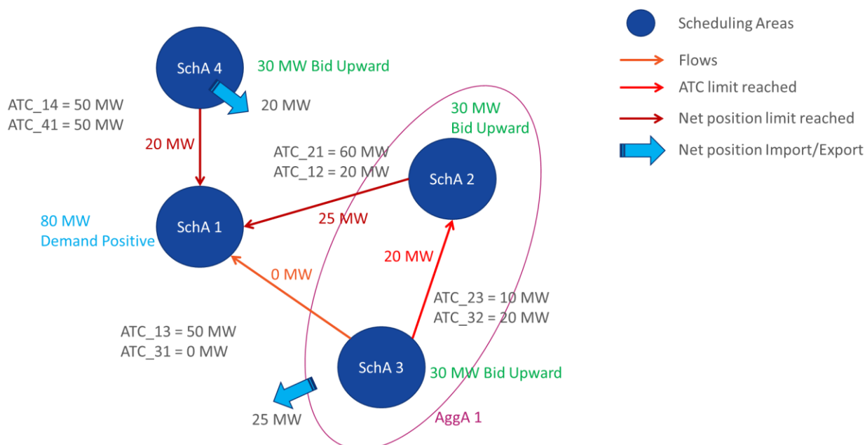
Figure 12: Feasible flow solution with net position limit
