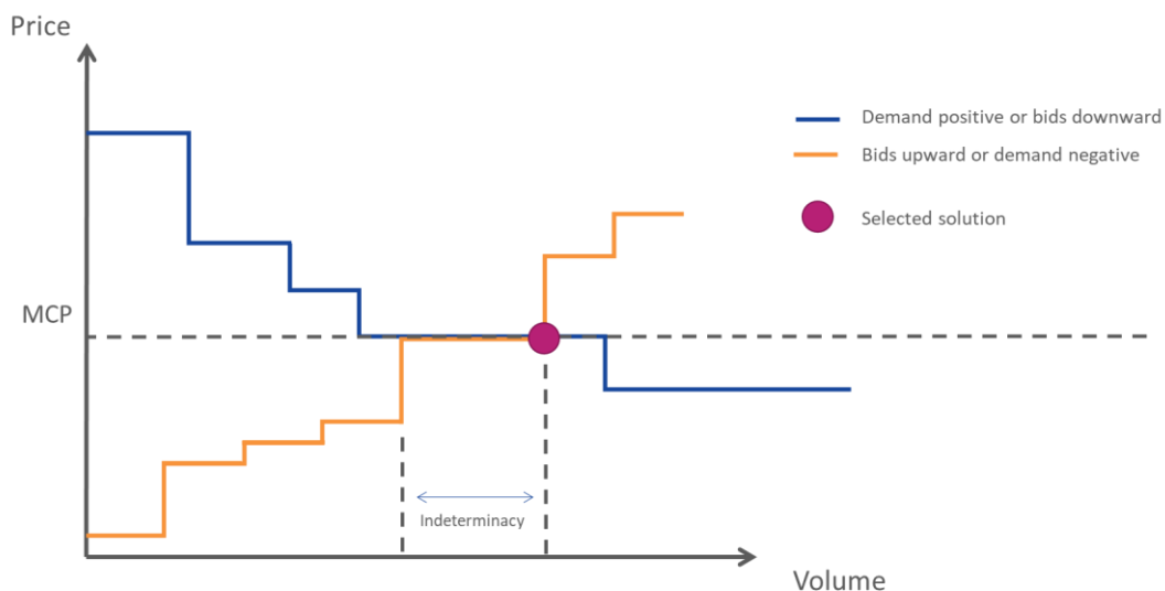
Figure 23: Volume indeterminacy
